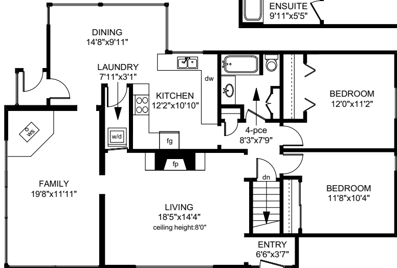
UNIT 1175/ MAIN FLOOR 1412 SQ.FT
